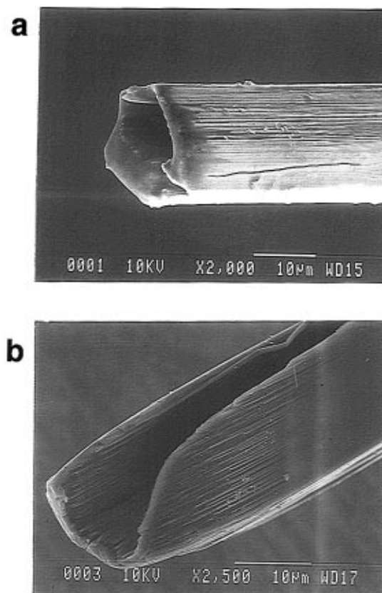
Figure 2. Scanning electron micrographs of [\text{Pt}^{\text{I}}(\text{bpy})_2](\text{NO}_3)_2 \cdot 2\text{H}_2\text{O} showing (a) the near-hexagonal shape of a crystalline needle and (b) the hollow nature of a damaged needle.
