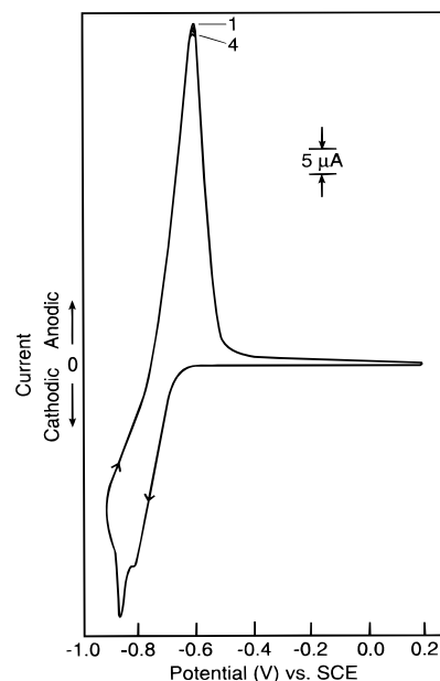
Figure 1. Cyclic voltammograms of 10 -3 M [Pt II (bpy) 2 ] 2+ in 0.1 M Na 2 SO 4 with an ITO electrode; scan rate of 100 mV/s.
